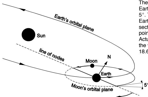
Figure 1.8.1. The orbital motions in the Sun-Earth-Moon system.
