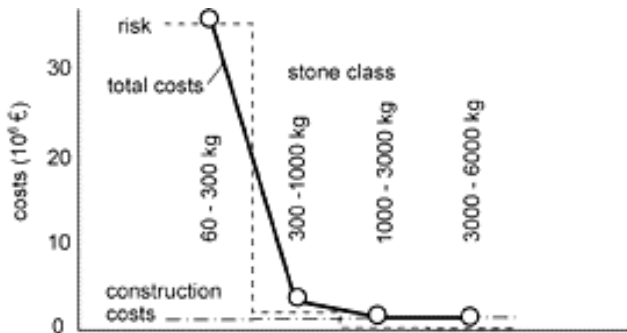
Figure 10-9 Risk and costs for various top layers
