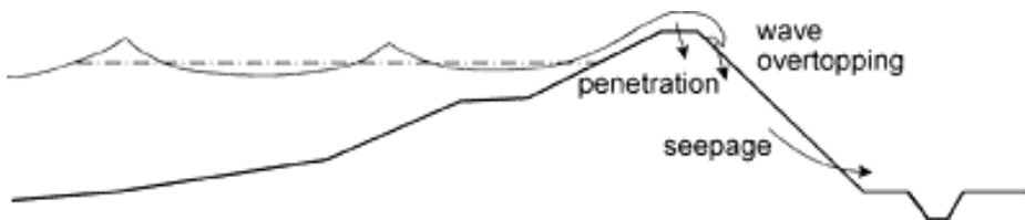
Figure 10-21 Collapse of dike due to micro-instability
