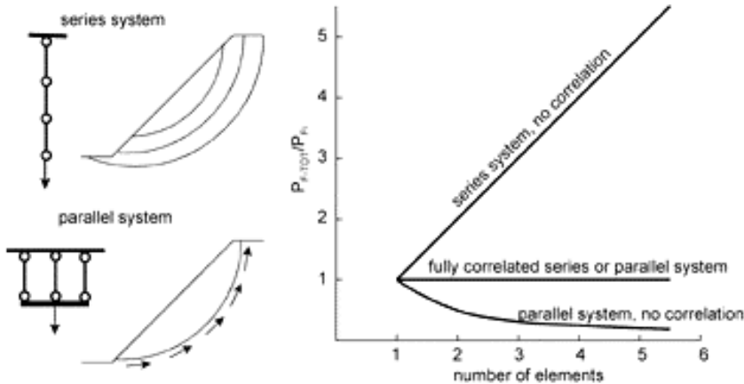
Figure 10-16 Series and parallel systems
